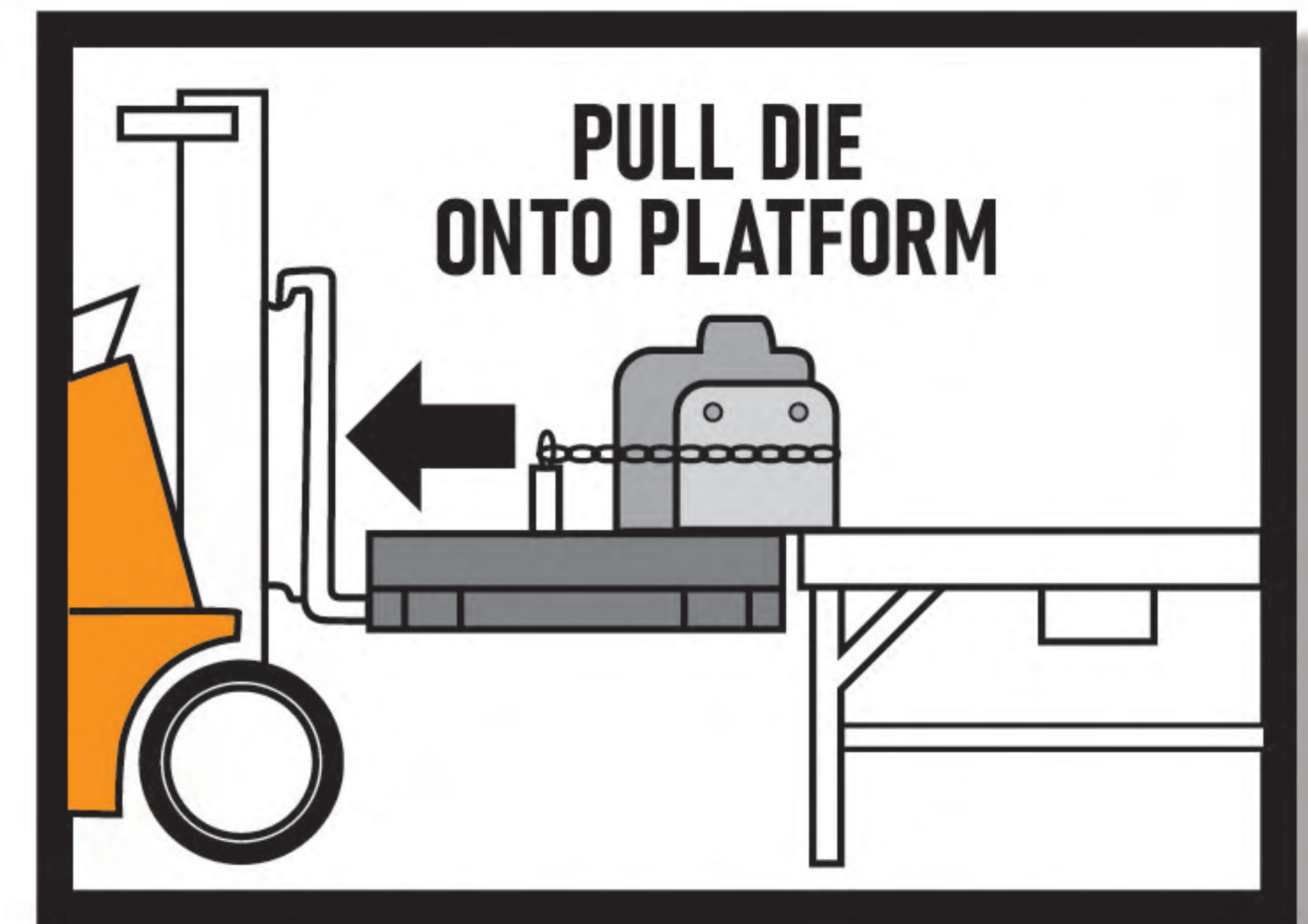
To pull die onto attachment - place chain around die, fasten it to draw bar, and then operate the control valve.
